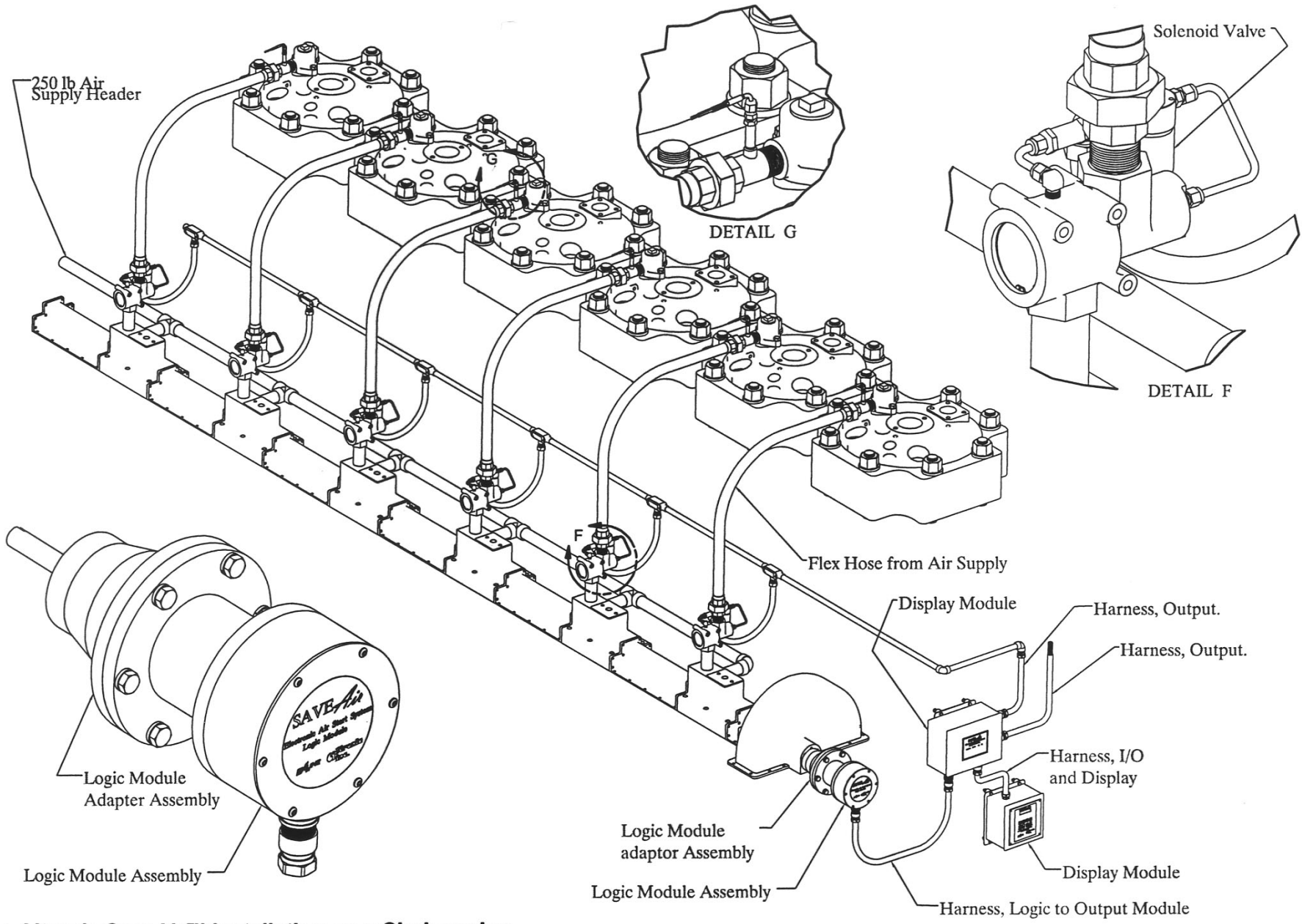
Typical Exline-Altronic SaveAir™ installation on a Clark engine.
