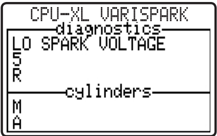
Low spark demand condition on cylinder 5R; often caused by a shorted spark plug or shorted secondary wire.
