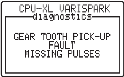
Zero gear-tooth pulses are seen between two reset pulses.
