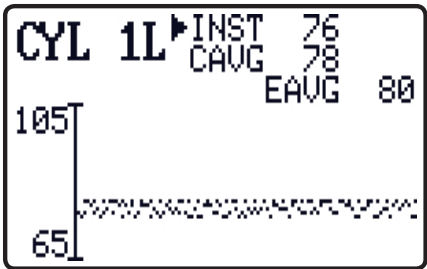
Spark diagnostics directly indicate breakdown voltage required. In this case, the cylinder average breakdown voltage (CAVG) required is 78, which indicates that the demand is 7.8kV
