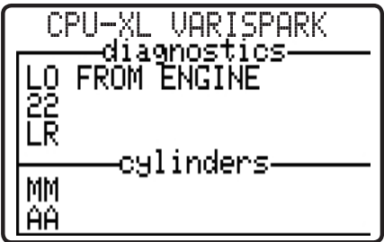
Condition detected where the average value of 2L and 2R is significantly lower than the average of other cylinders on the engine. HI FROM ENGINE diagnostic is also available.
