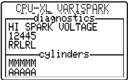
High spark demand condition on cylinders 1R, 2R, 4L, 4R, and 5L ; often caused by worn spark plugs.
