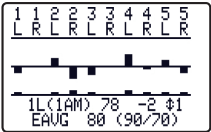
Enhanced display allows the user to monitor all cylinders simultaneously.
